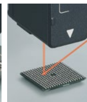
Diffuse reflection
